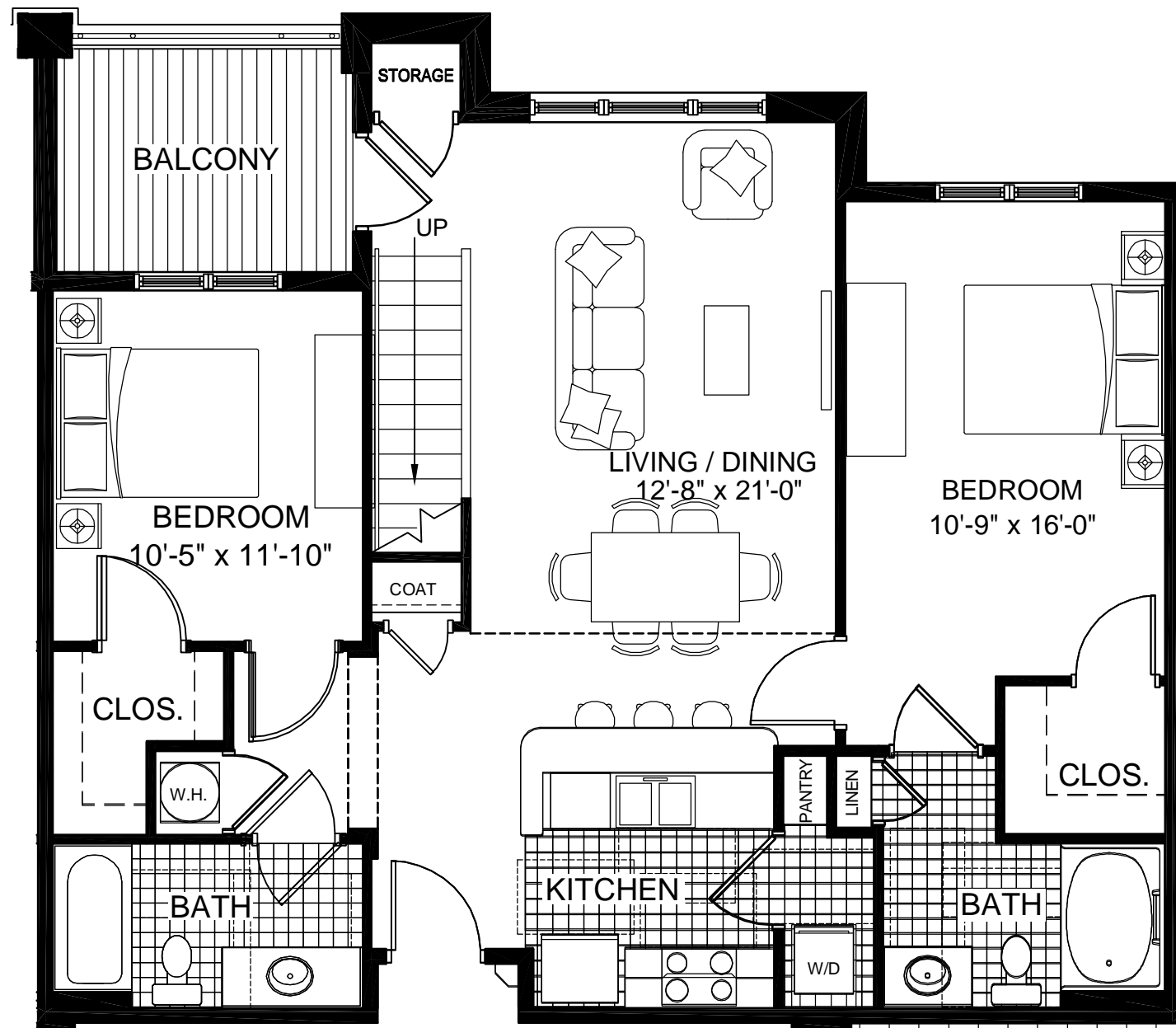
MAIN LEVEL
